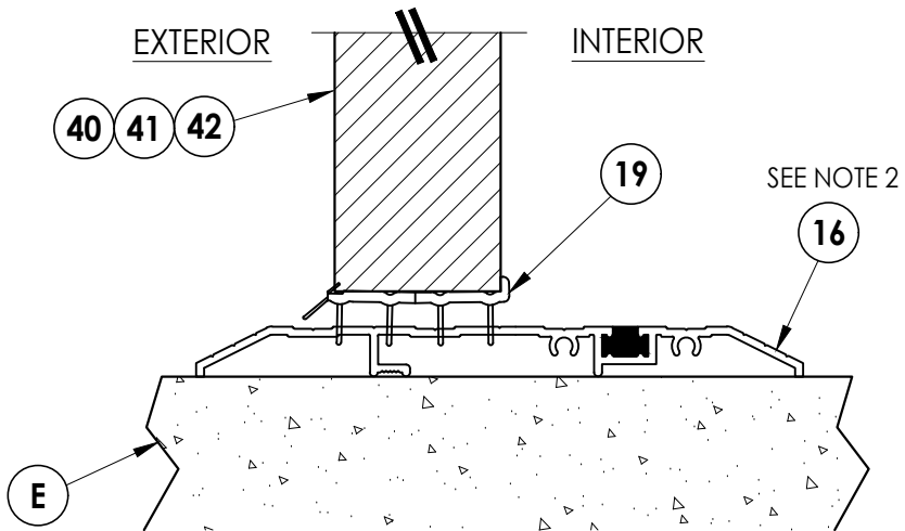
3 7 VERTICAL CROSS SECTION Public Access Sill
